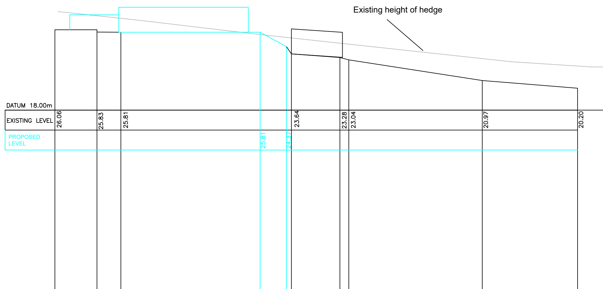
SECTION 2-2
