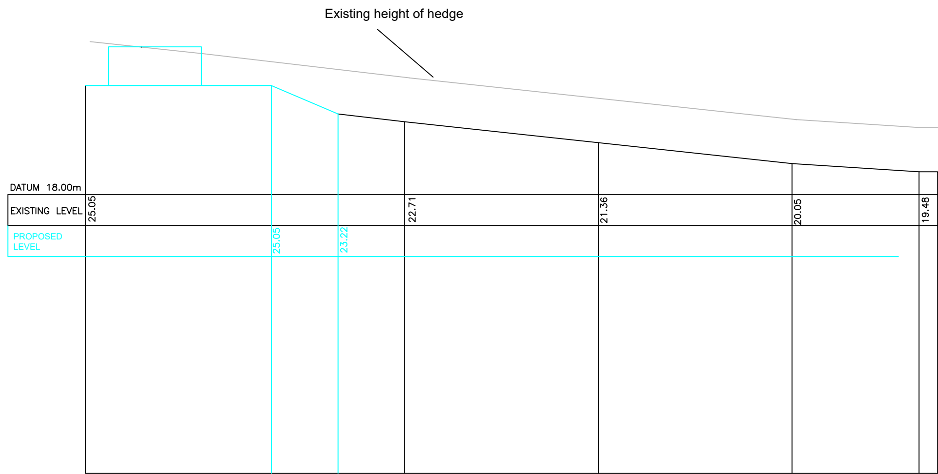
SECTION 1-1
