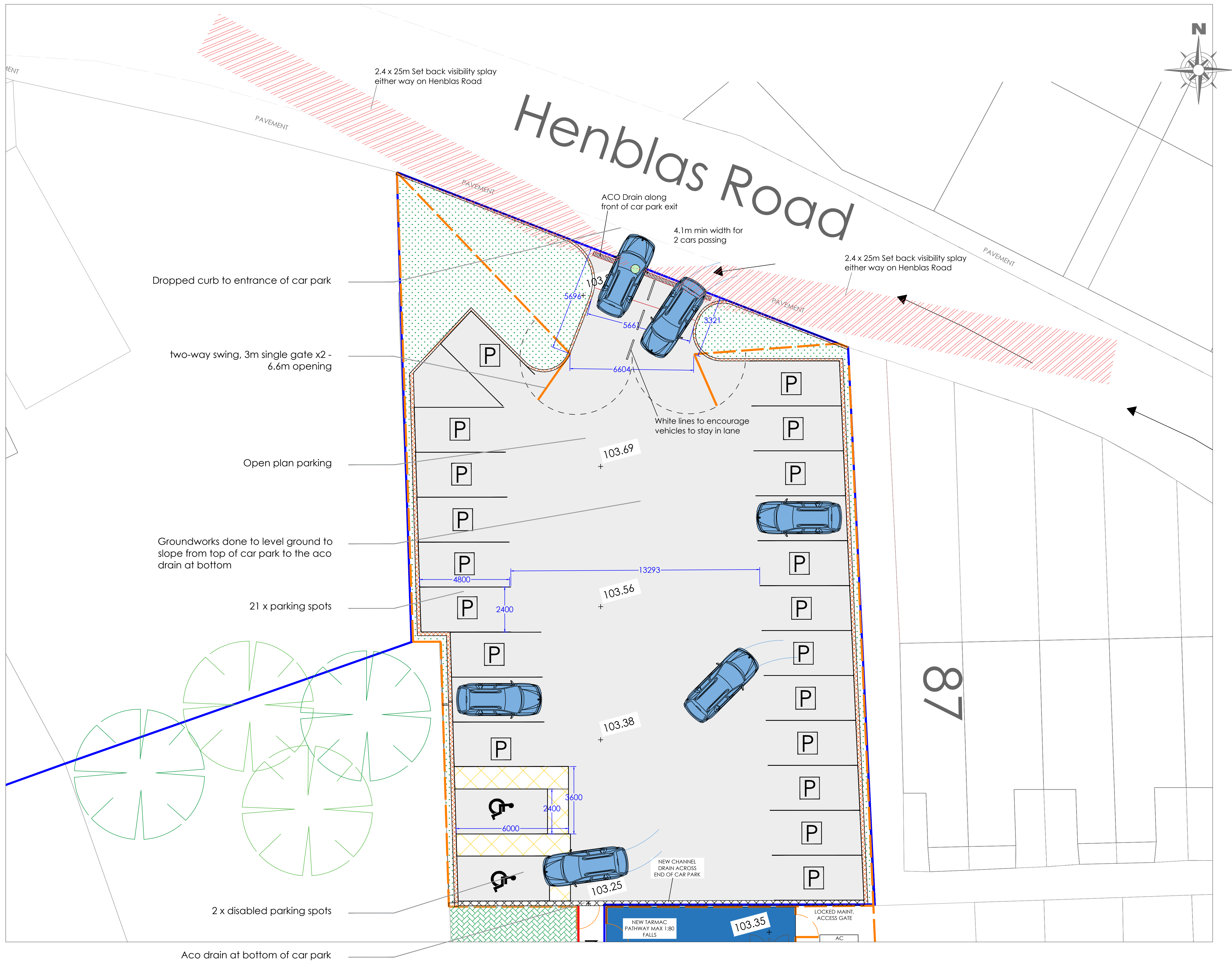
Car park layout OPTION C
