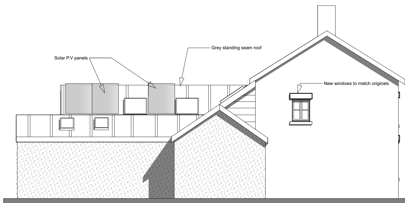
West Elevation
