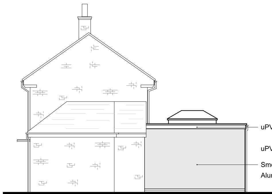
Proposed Side Elevation View A - 1:100
