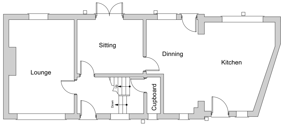
Existing Ground Floor Plan 1:100
