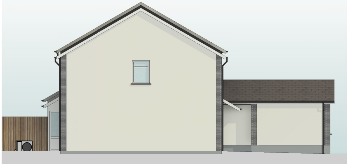
2 South East Elevation
