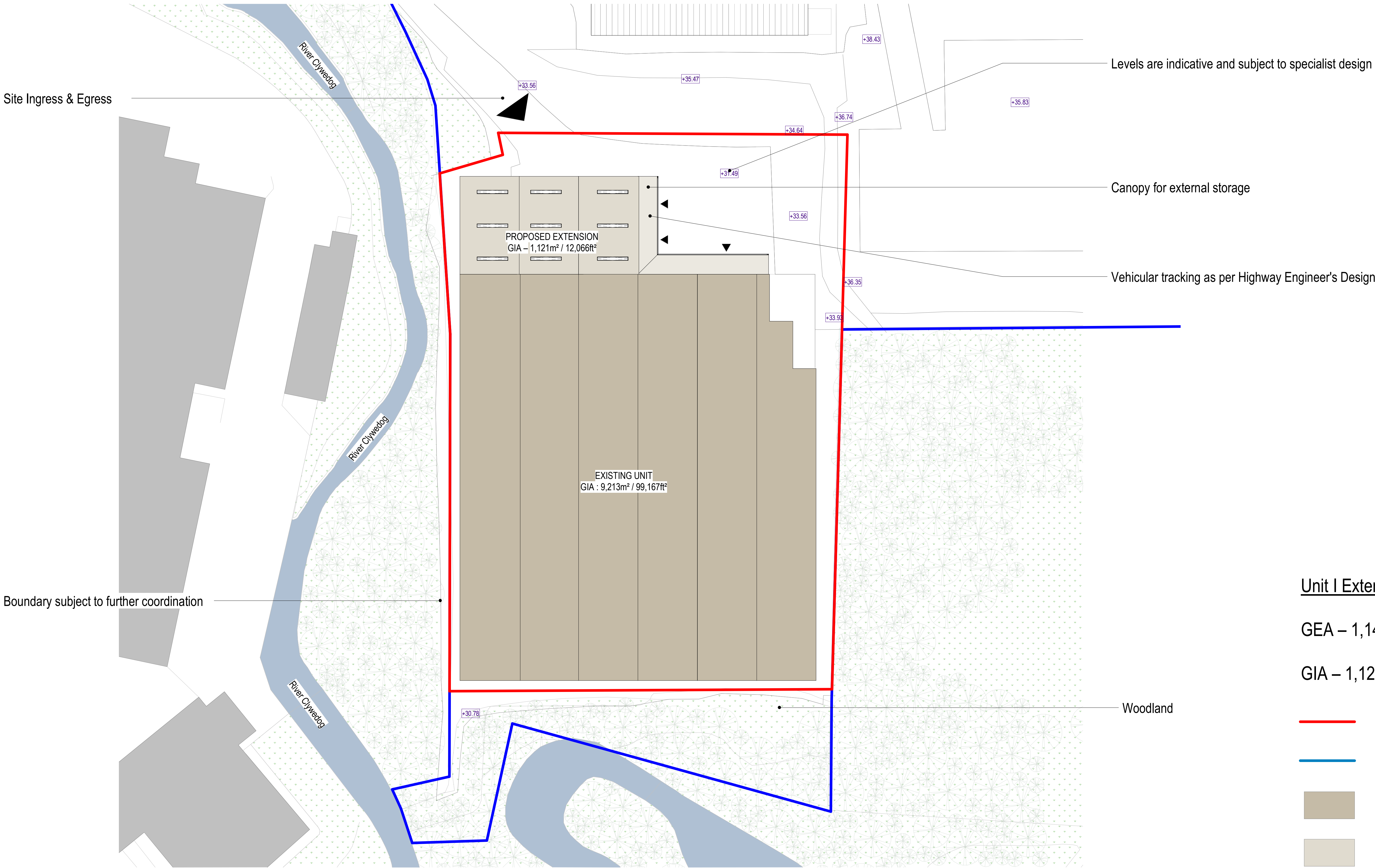
1 Proposed Site Plan (Unit I Extension) 1 : 500
