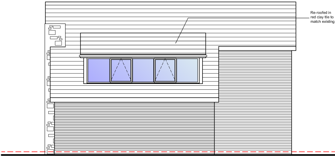
SIDE ELEVATION
