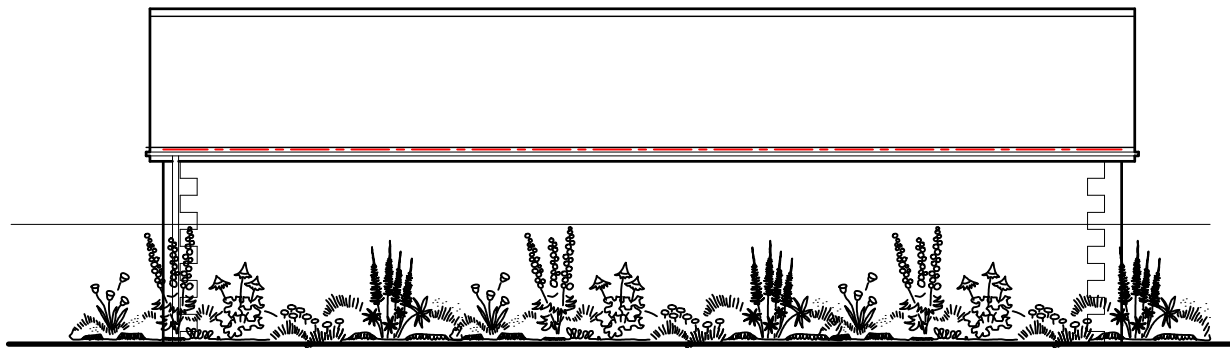
Rear elevation 1:100
