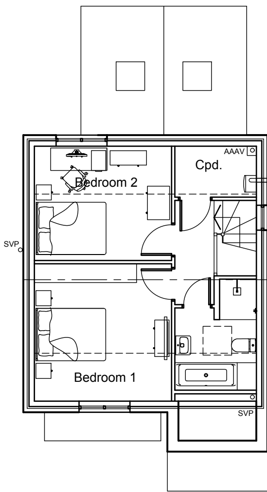
2. First Floor Plan
