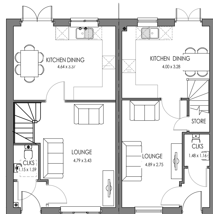
HIGHFIELD AS GROUND FLOOR
