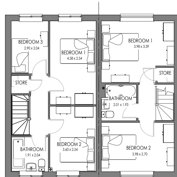
HIGHFIELD AS FIRST FLOOR
