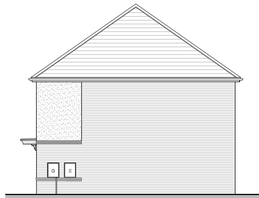
OAKLEY OPP SIDE ELEVATION
