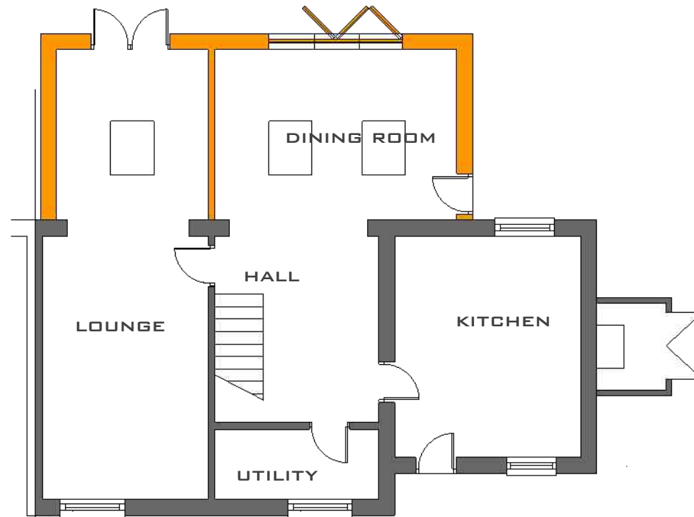
A 7 1:100 Floor Plan
