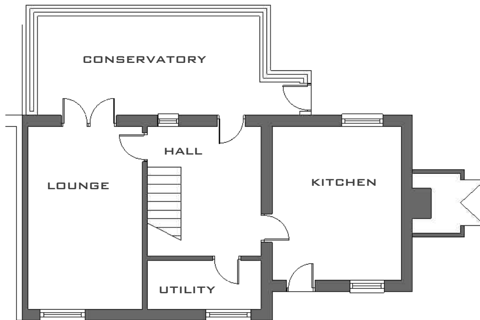
A 3 Floor Plan 1:100
