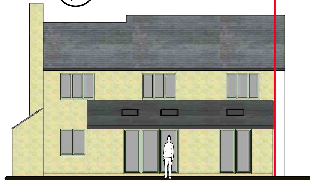
A 9 1:100 Rear Elevation
