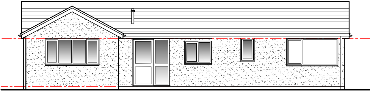
Front elevation 1:100
