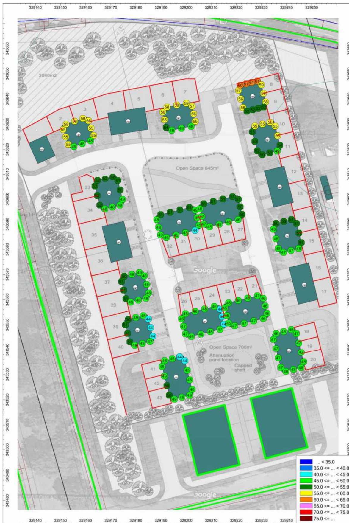
Figure D.7 – Proposed development - Predicted façade dB L_{Aeq,16hr} exposure levels – Daytime (07:00 – 23:00) – First floor
