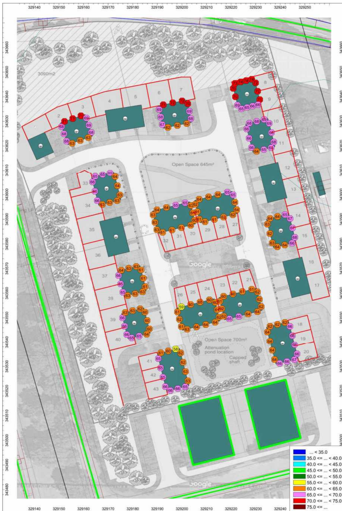
Figure D.11 – Proposed development - Predicted façade dB L_{A_{\text{max}}} exposure levels – Night-time (23:00 – 07:00) – First floor
