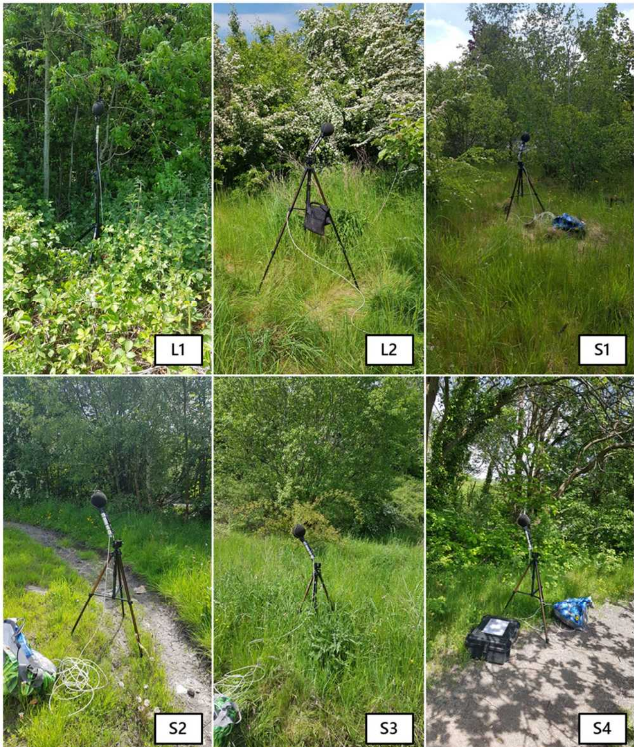
Figure B.2 – Photographs of the noise monitoring positions
