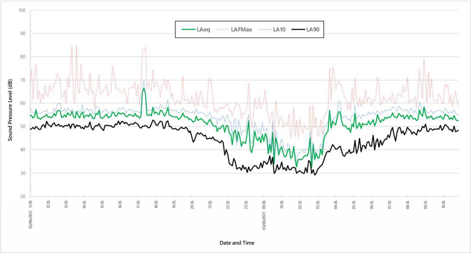
Figure 4.1 – Graph of measured noise levels at position L1
