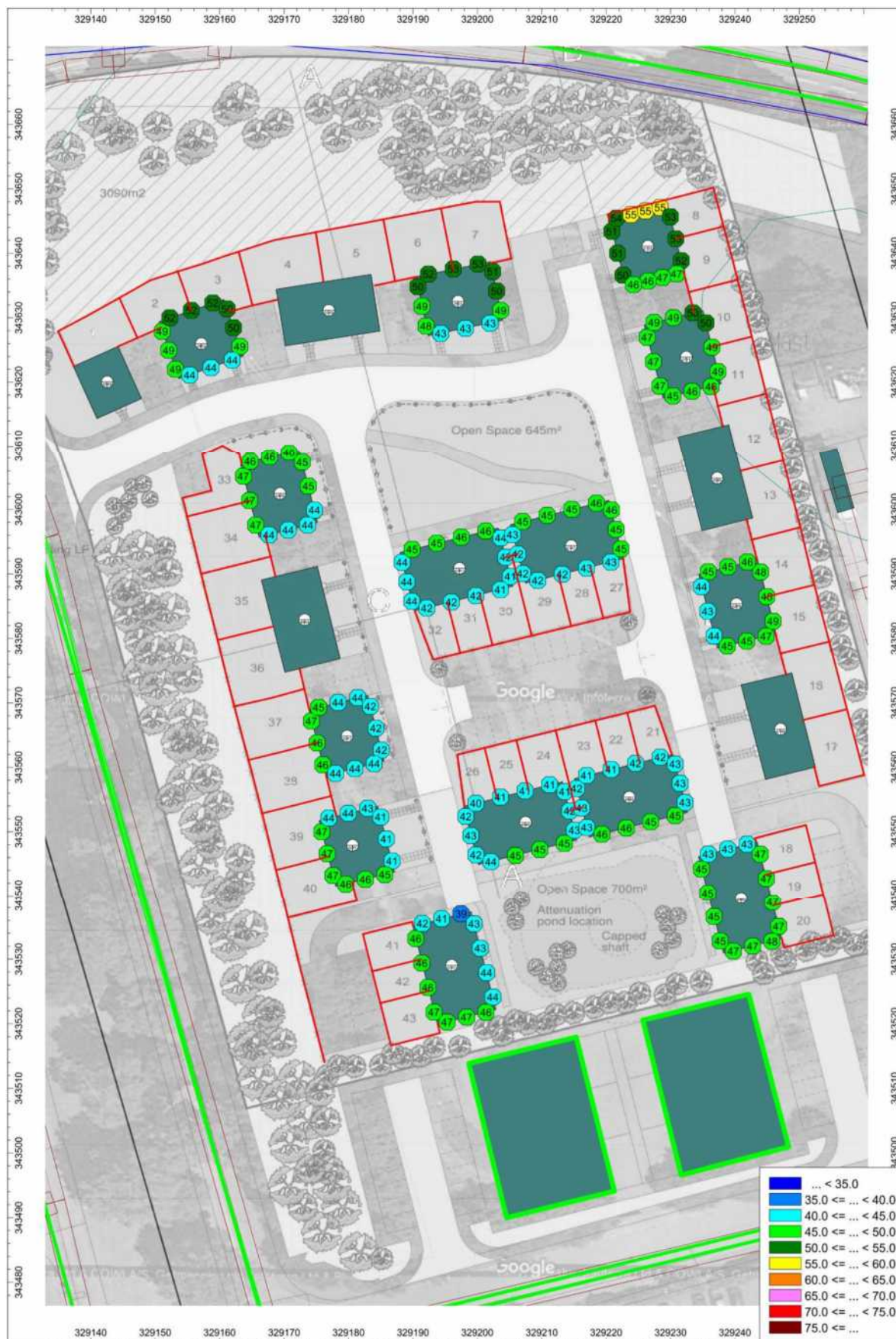
Figure D.9 – Proposed development - Predicted façade dB L_{Aeq,8hr} exposure levels – Night-time (23:00 – 07:00) – First floor
