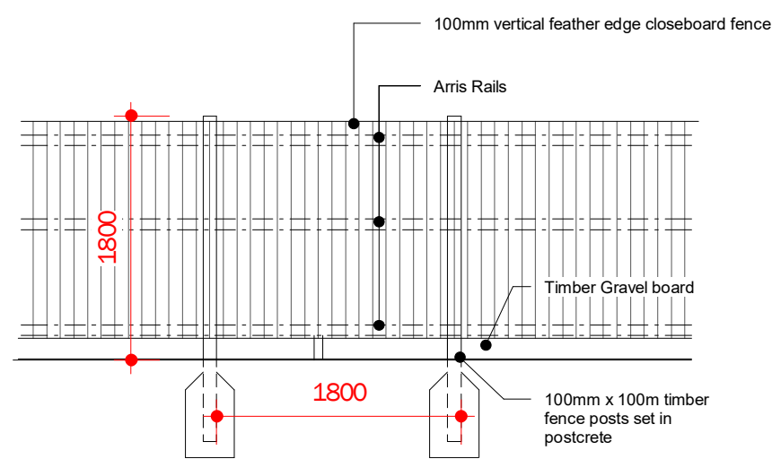
F1 - Boundary Treatment 1.8m Feather edge Scale: 1:50
