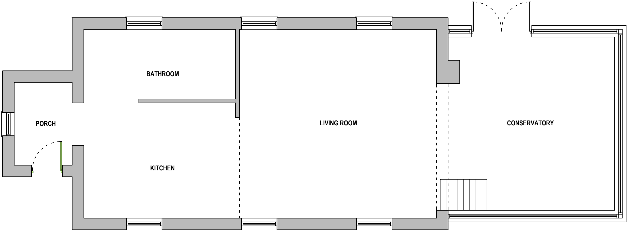
EXISTING GF LAYOUT
