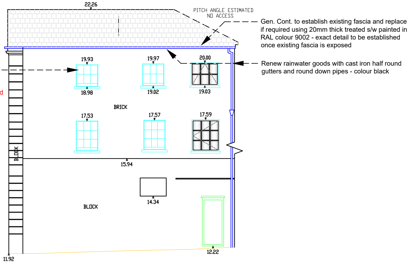
38 Henblas Street - Proposed Side Elevation
