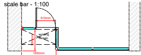
38 Henblas Street - Proposed Plan
