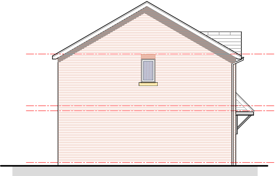
Plot 3 Side Elevation
