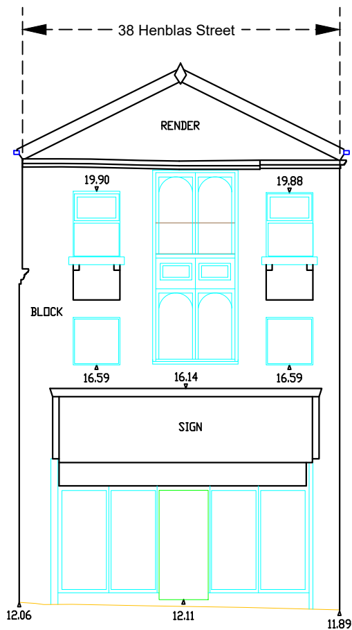
38 Henblas Street - Front Elevation
