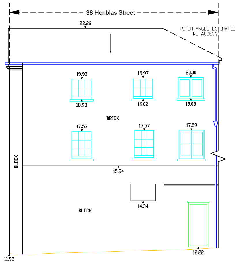
38 Henblas Street - Side Elevation
