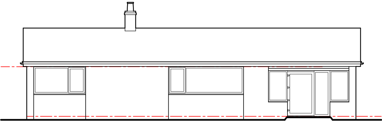
Rear elevation 1:100
