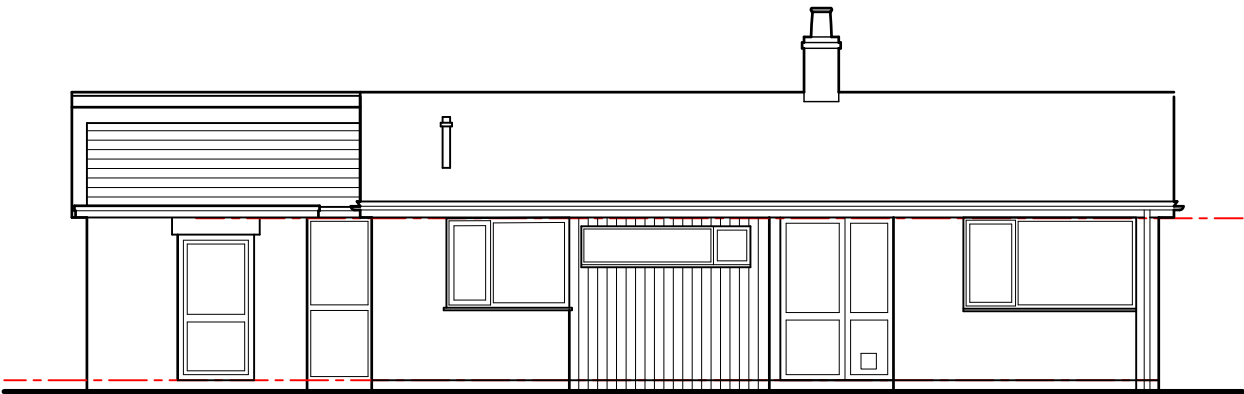
Front elevation 1:100
