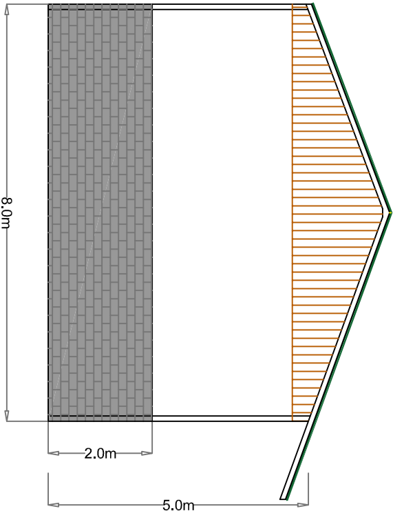
Side Elevations
