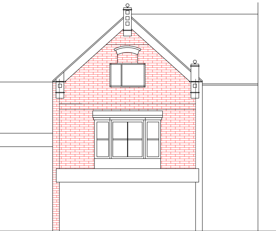
PROPOSED front elevation (NO CHANGE)
