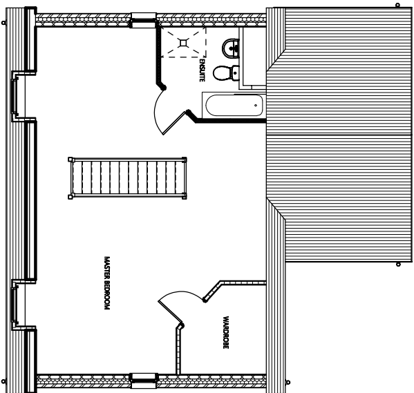
02 LOFT STRUCTURAL
