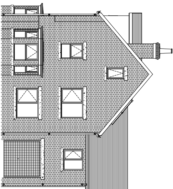
RH GABLE ELEVATION
