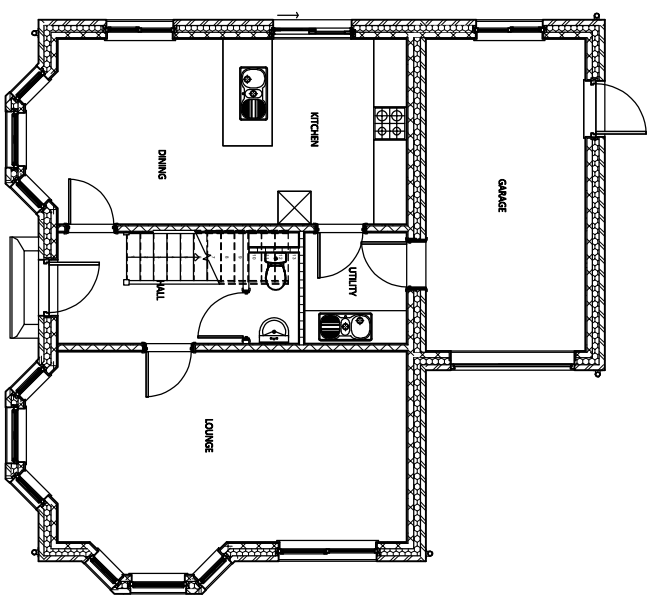
00 GROUND FLOOR STRUCTURAL
