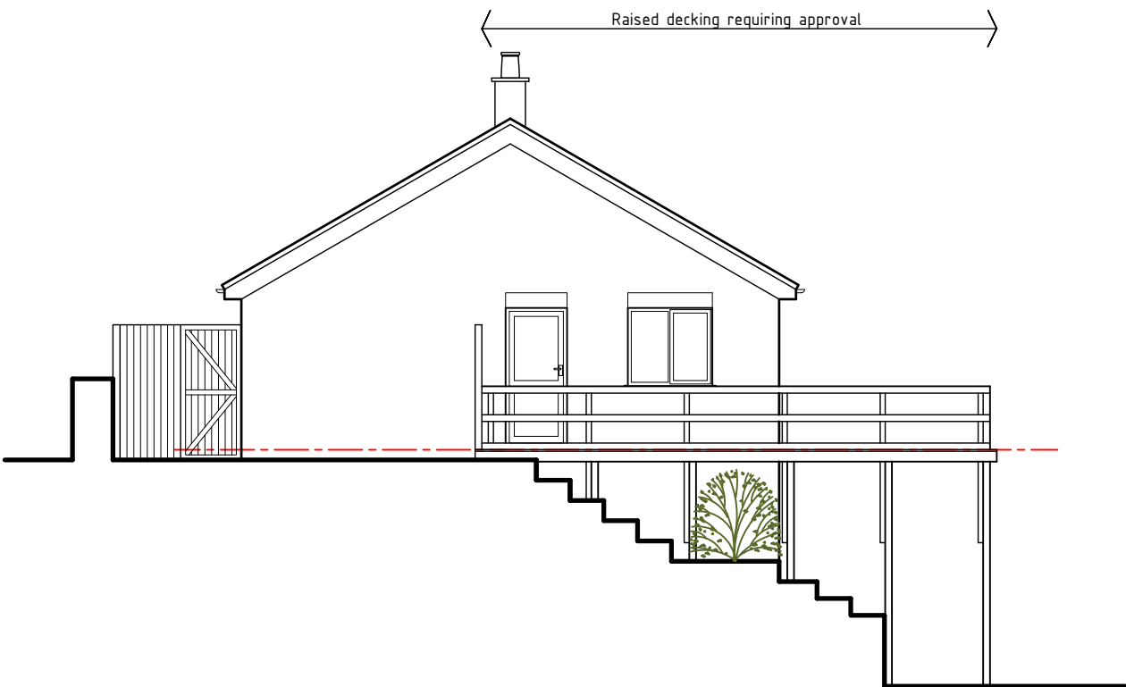
Side-01 elevation 1:100
