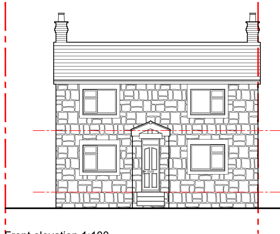
Front elevation 1:100
