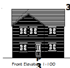
Front Elevation 1:100
