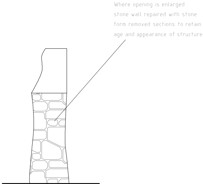
End Detail 1:25
