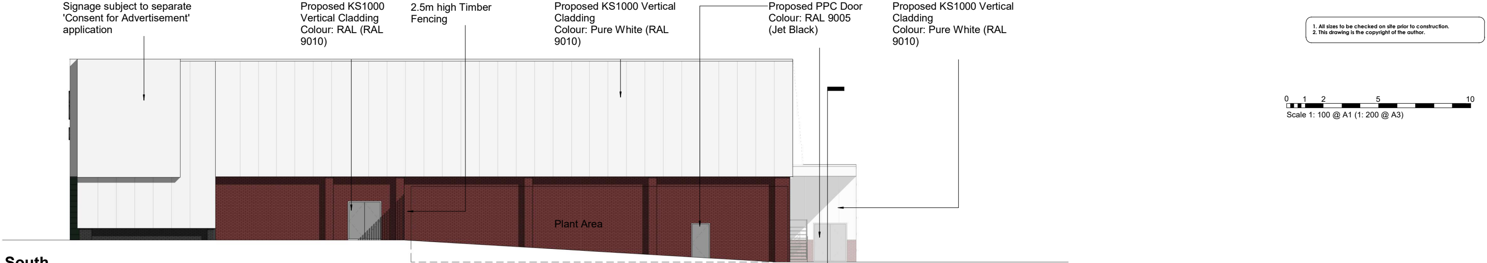
South 1 : 100
