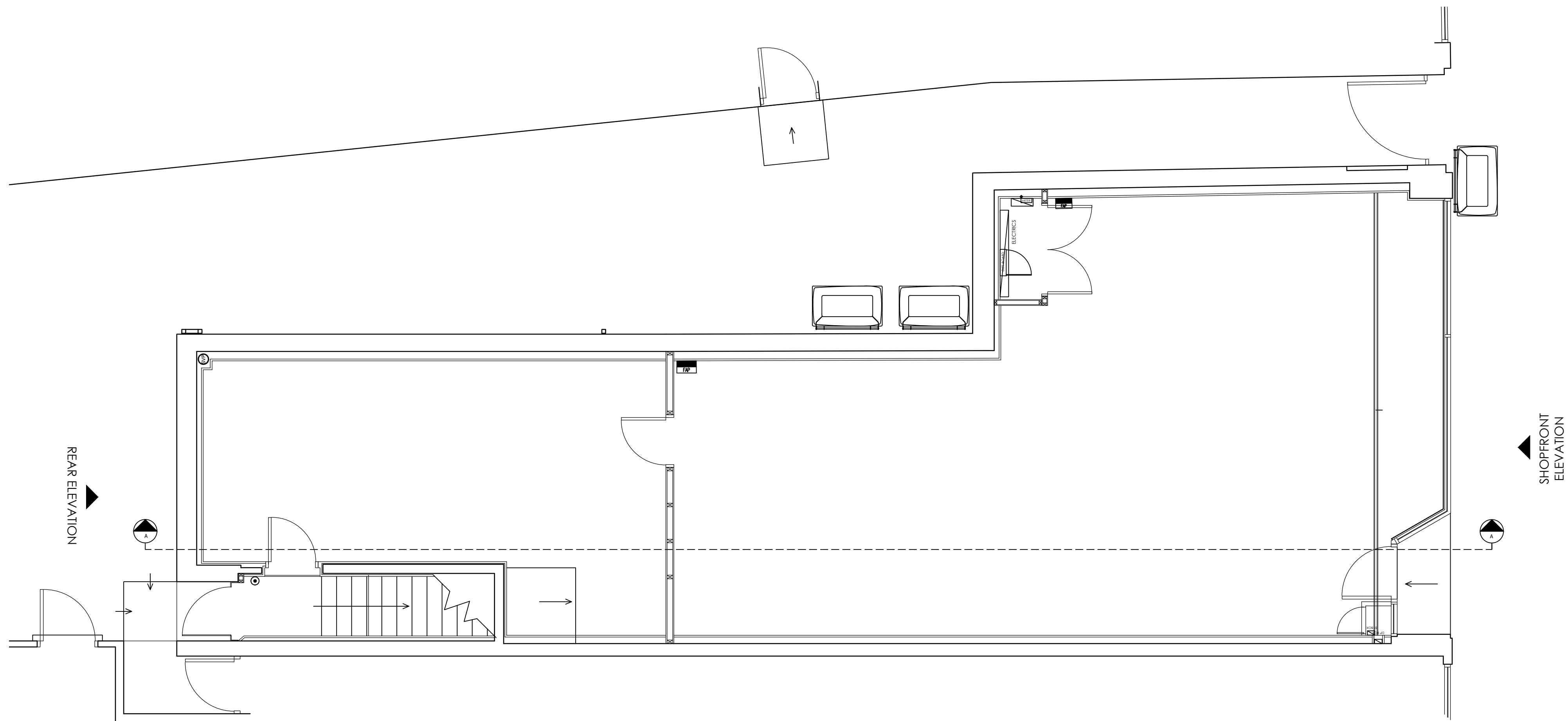
EXISTING GA PLAN - FIRST FLOOR (1:50)
