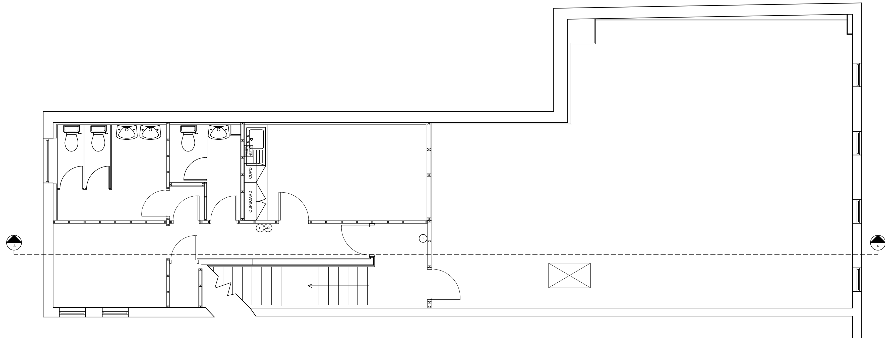
EXISTING GA PLAN - FIRST FLOOR (1:50)
