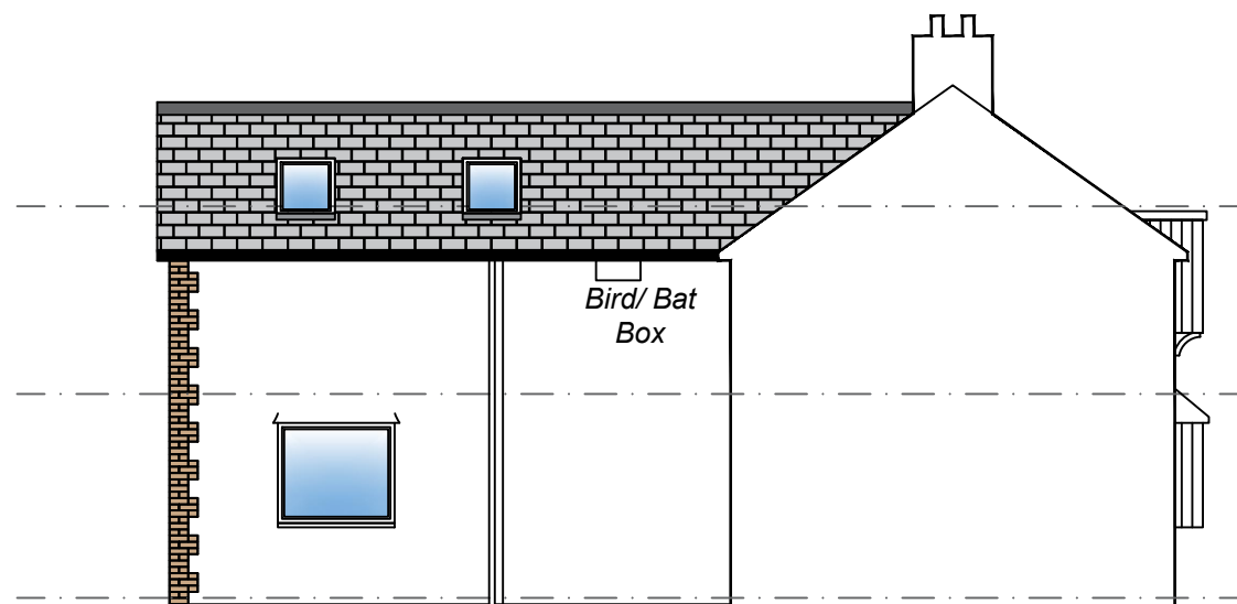
SIDE ELEVATION
