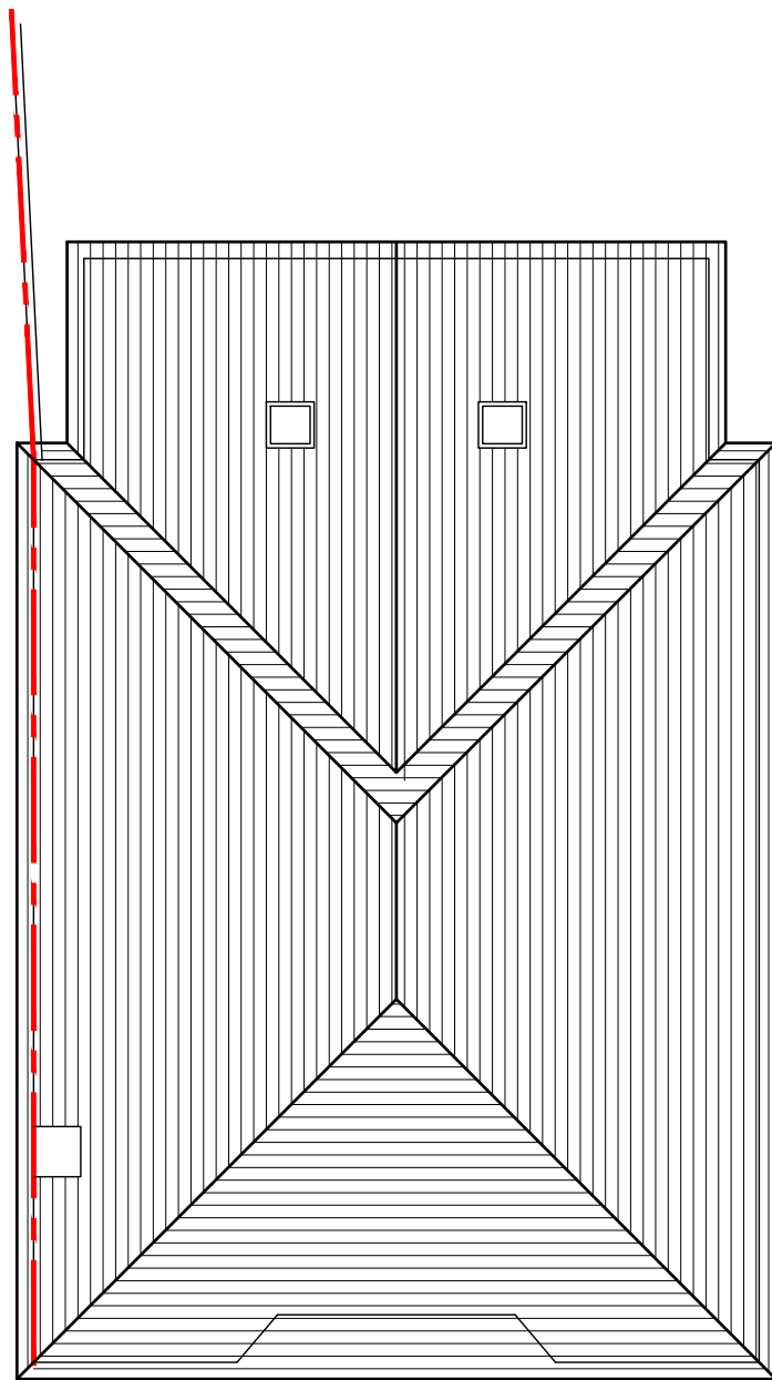
Roof Plan 1:100
