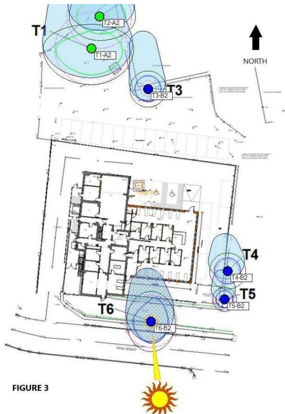
Figure 3: June 13:00hrs: shows partial extension (approximately 10%) of shadow over the roof of the proposal where the photovoltaic panels (PV) will be sited. T6 will be in full leaf during the month of June, however the majority of PV panels are unlikely to be shaded. Figure 3A: June 13:00hrs: showing T6 shadow with a 20% crown reduction.
