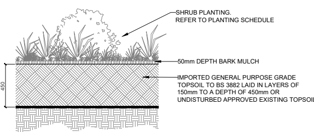
02 SHRUB PLANTING SCALE: 1:40 @ A1
