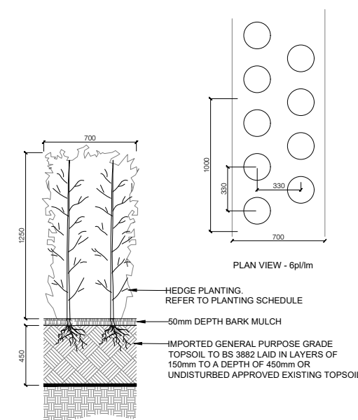
03 HEDGE PLANTING - STAGGERED DOUBLE ROW SCALE: 1:40 @ A1
