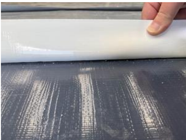
Double sided tape to joint
