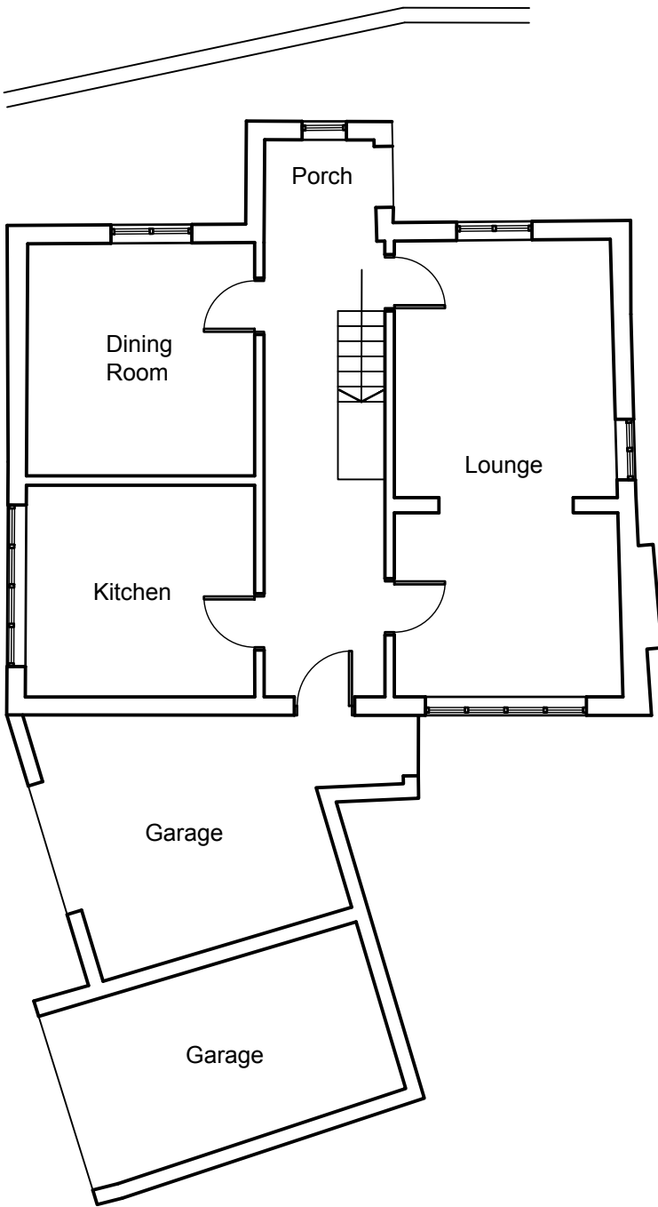
1. Ground Floor Plan - As Existing
