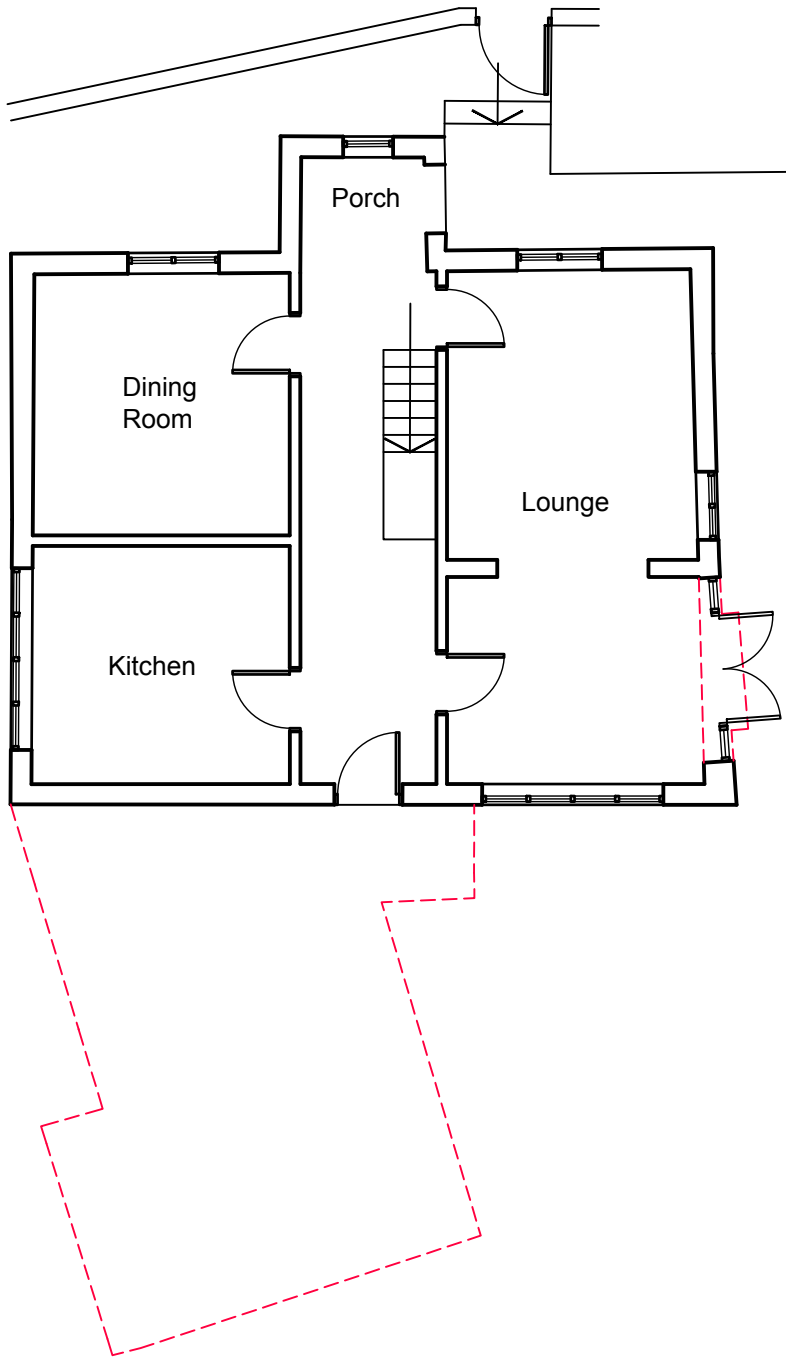
2. Ground Floor Plan - As Proposed
