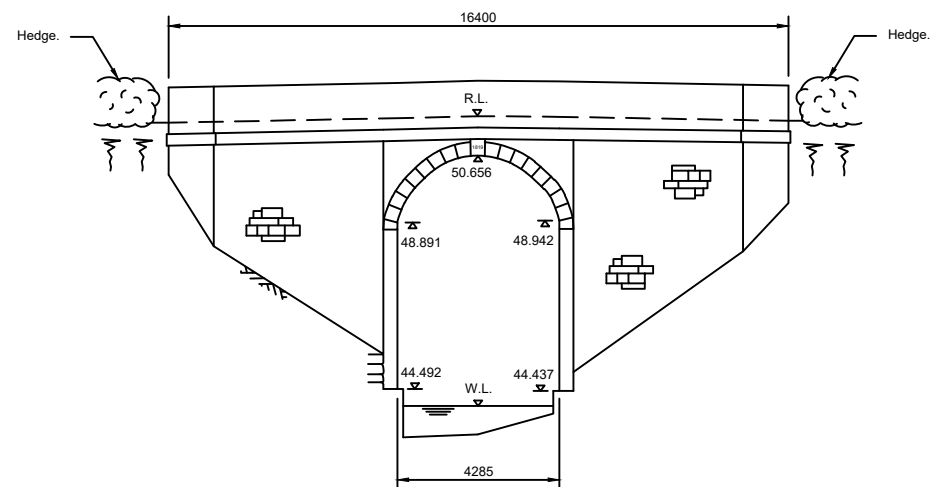
ELEVATION B - B Scale 1 : 100
