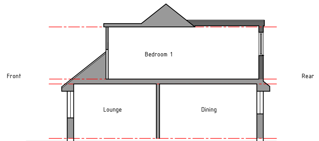
Typical Section 1:100 As Proposed
