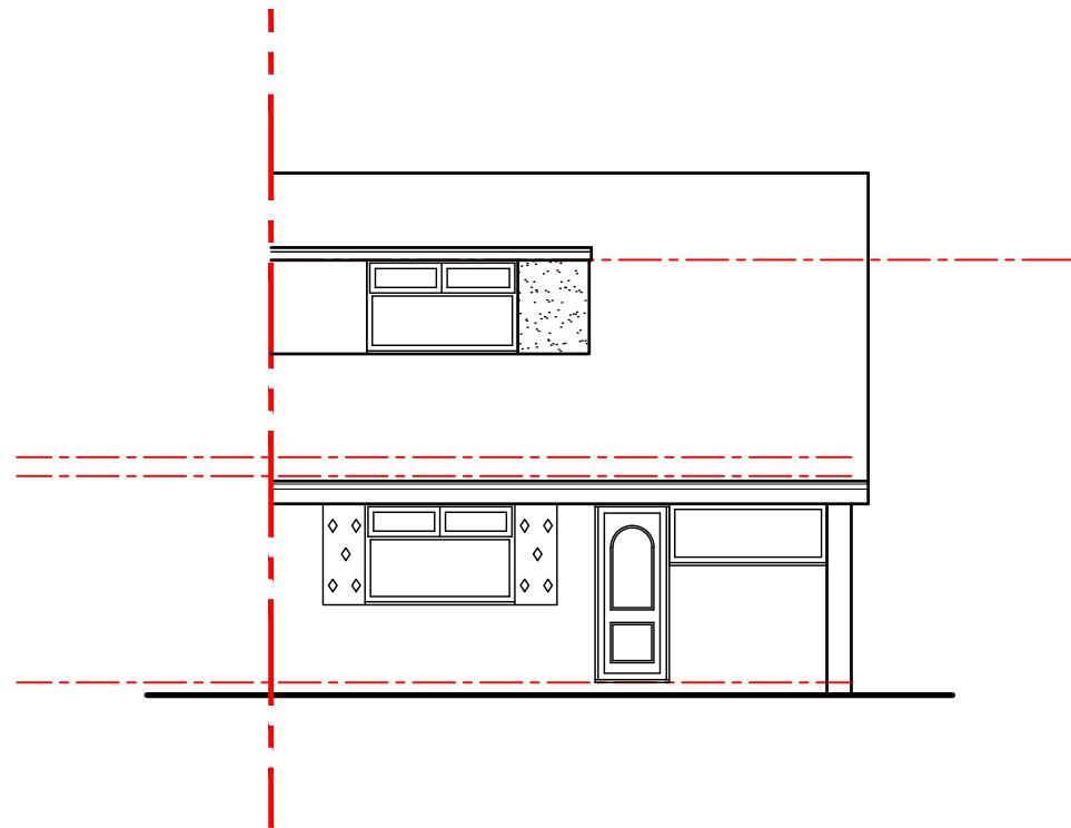
Front elevation 1:100
