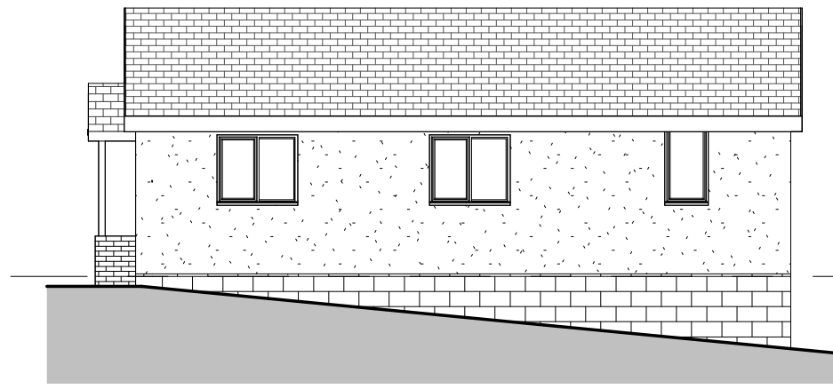
Side Elevation 1 : 100
