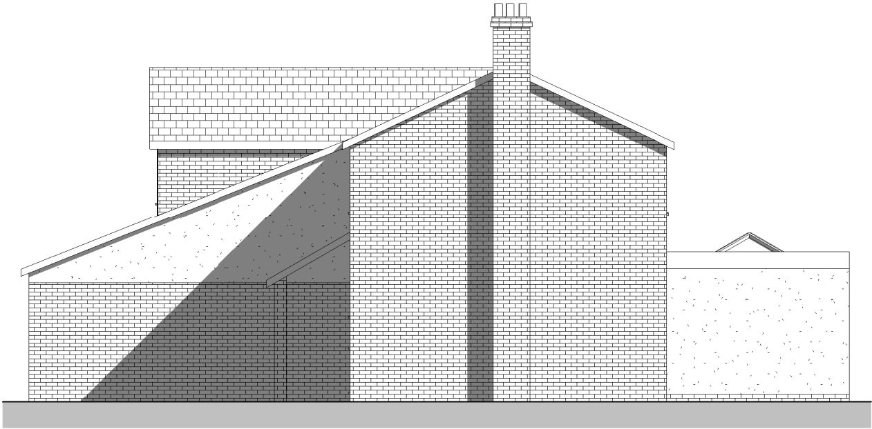
Side Elevation 1 : 100
