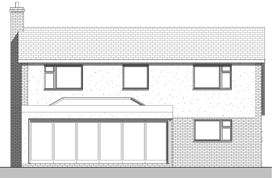
Rear Elevation 1 : 100
