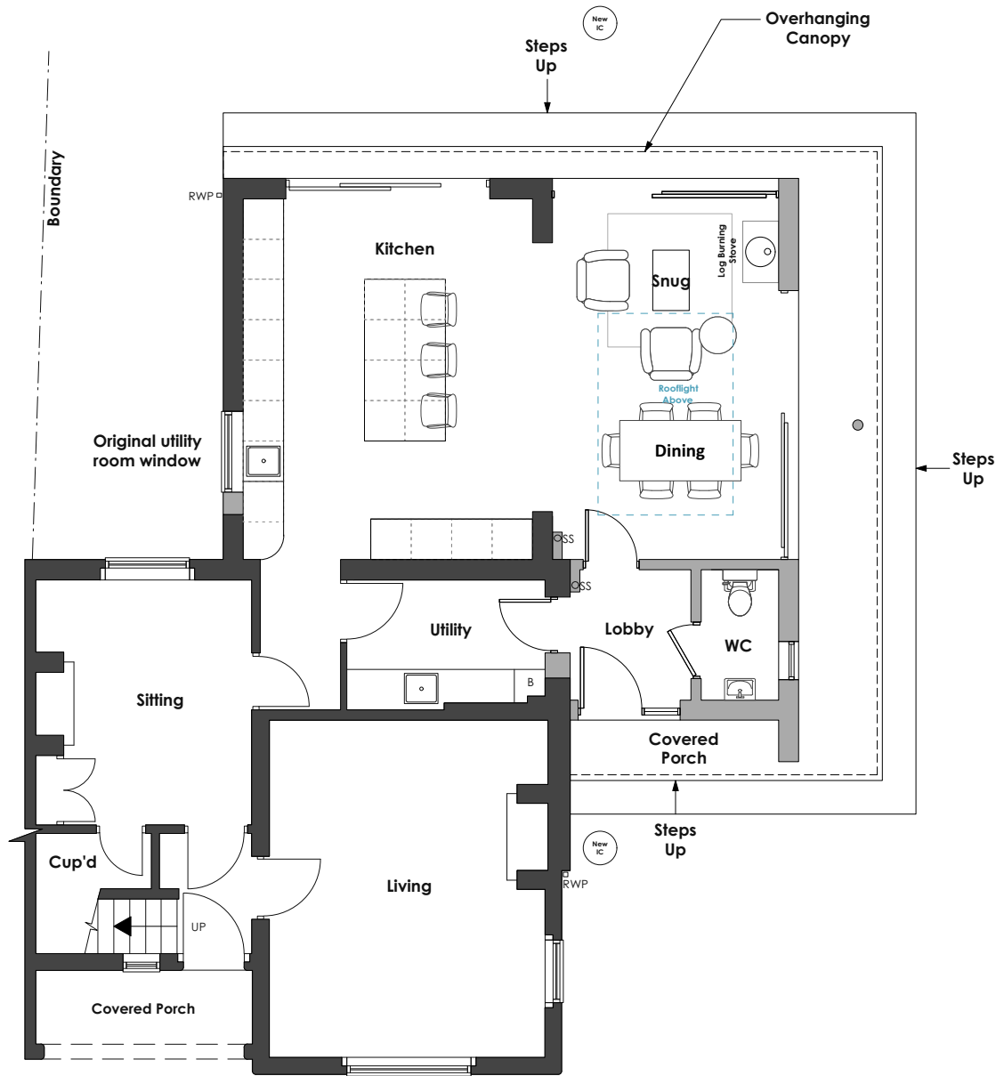
Proposed Ground Floor Plan 1:50
