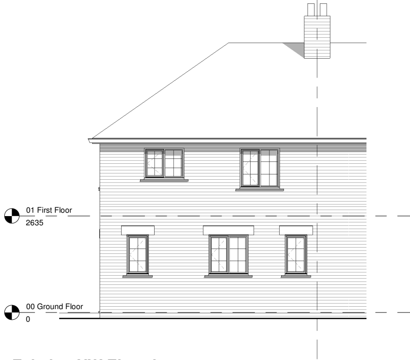
Existing NW Elevation 1 : 50
