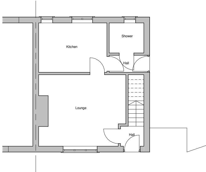
Existing Ground Floor Plan 1 : 50
