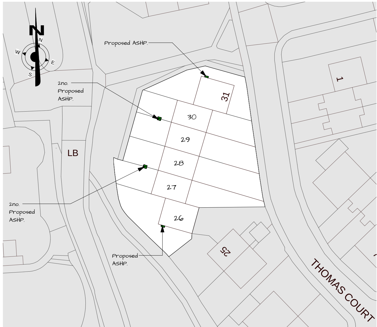
6 Block Plan
