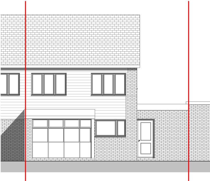
Rear Elevation 1 : 100
