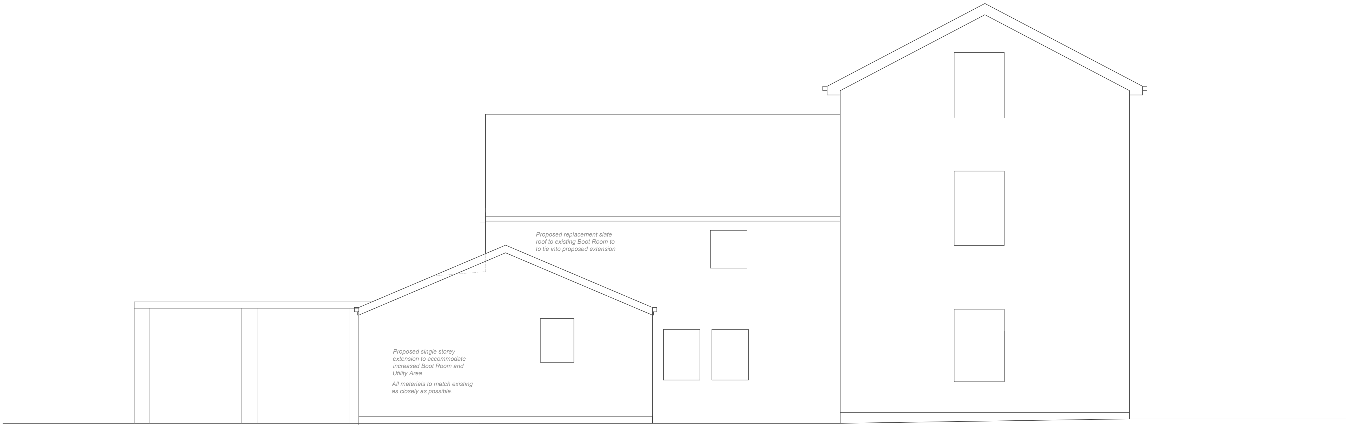
Side North Elevation (1:50)
