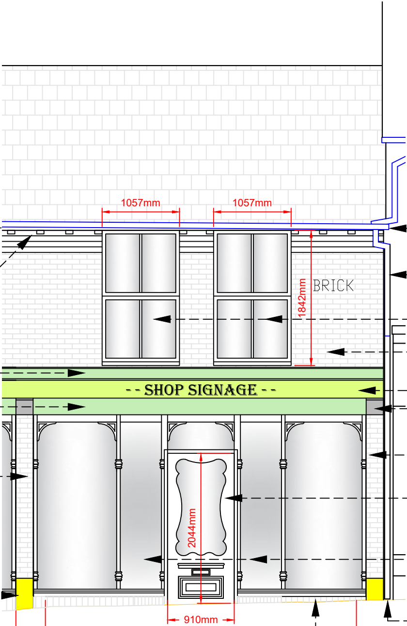
2 Henblas Street - Proposed Elevation
