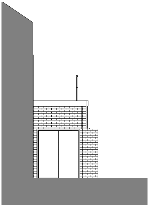
Front Elevation 03 1 : 100
