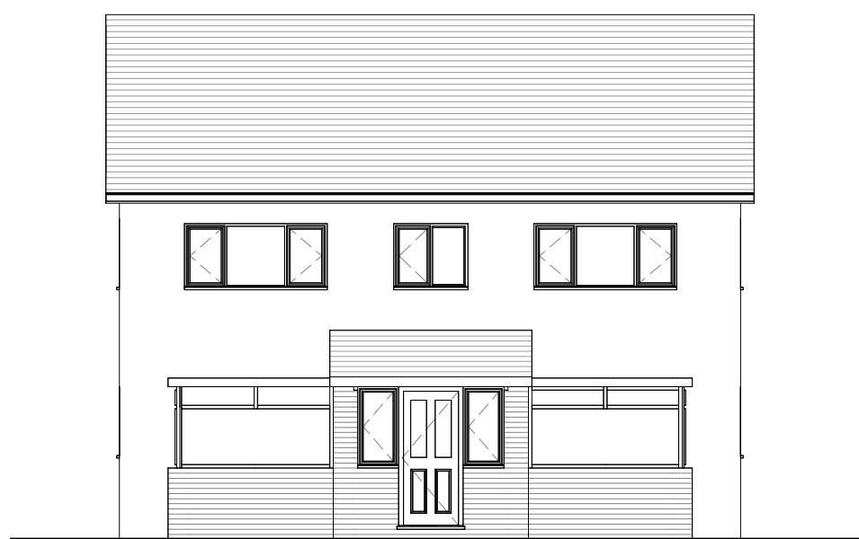
224 Holt Rd - West Elevation 1 : 100
