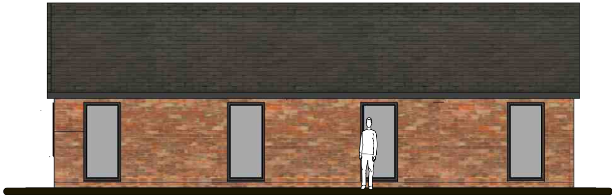
A 15 Front Elevation 1:100
