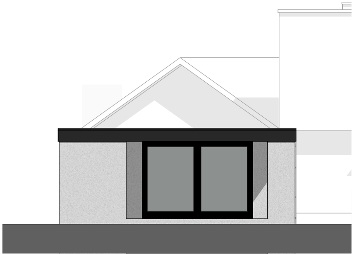
E6 - Garden Room Side Elevation 1:100
