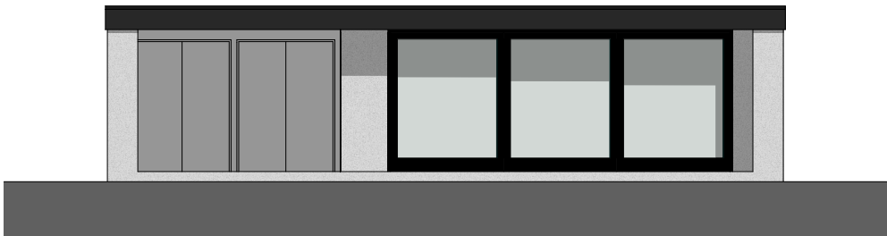
E5 - Garden Room Front Elevation 1:100
