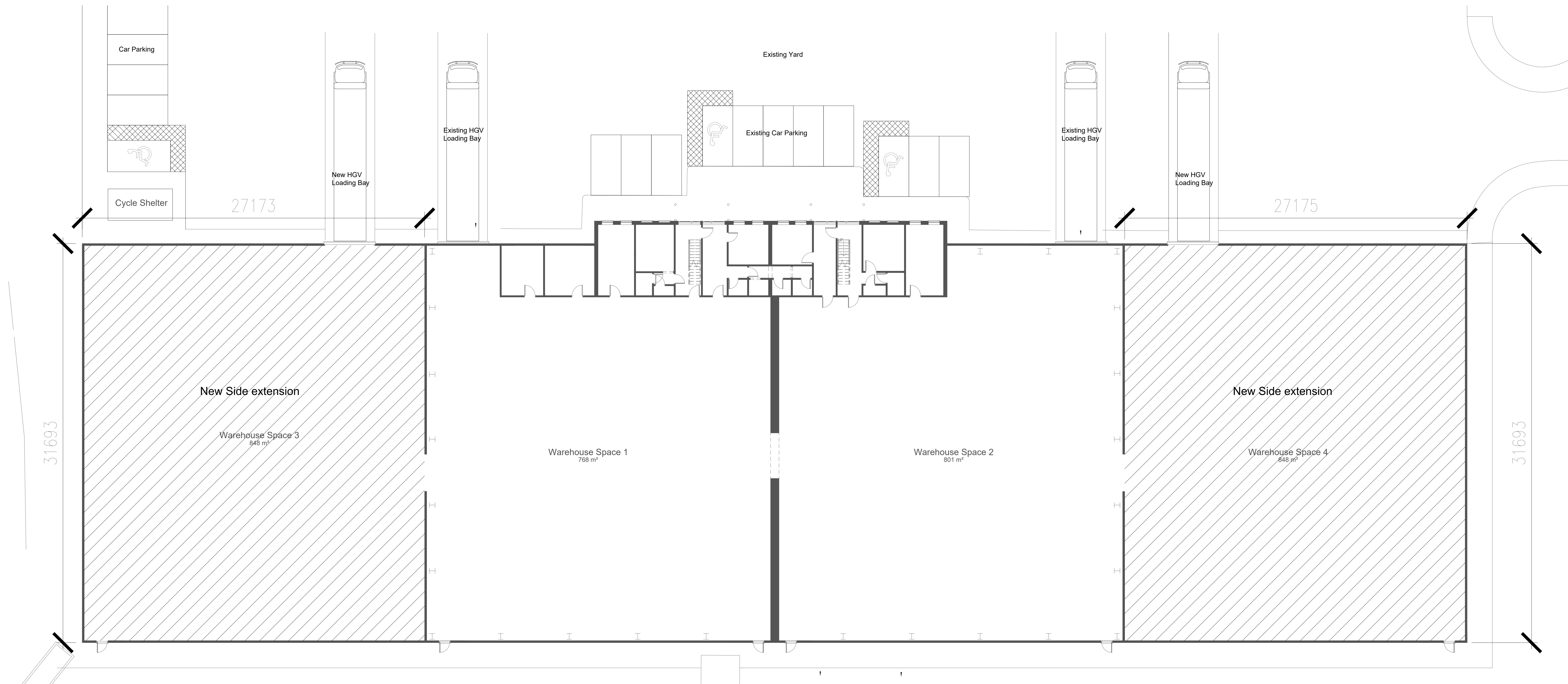
Proposed Ground Floor Plan
