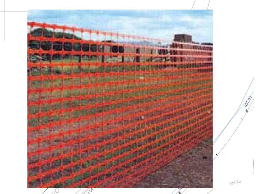
DETAIL 3 Euromesh plastic barrier fencing to hedgerow RPAs
